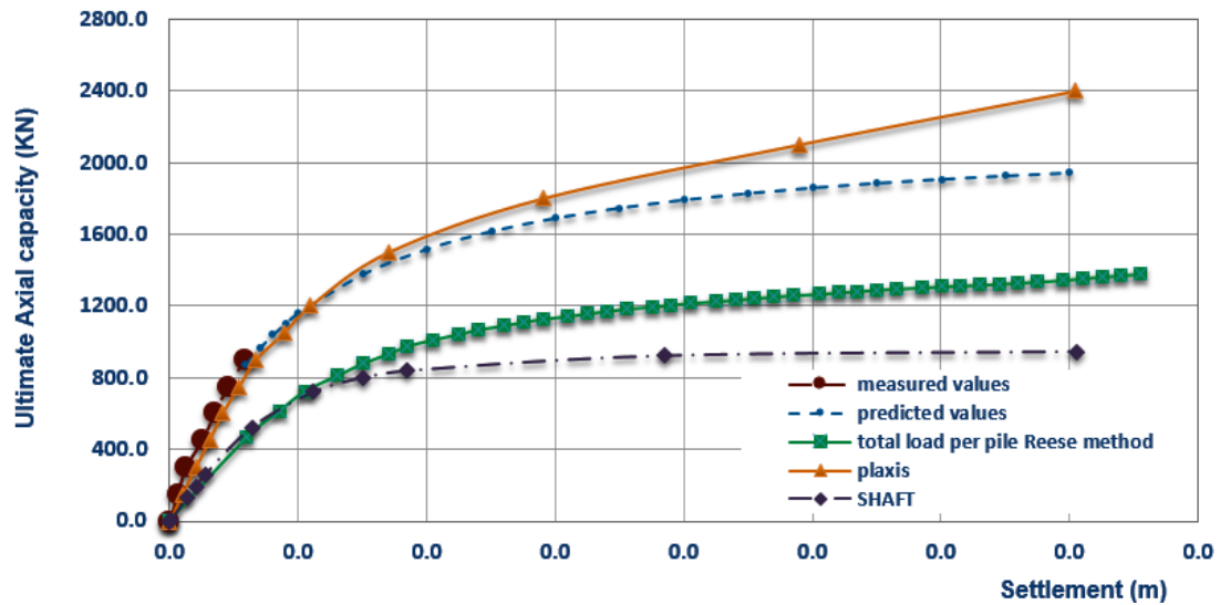
Figure 11: Load- settlement behavior of the pile model No (21) using different methods in a site at Qu-tour city.
