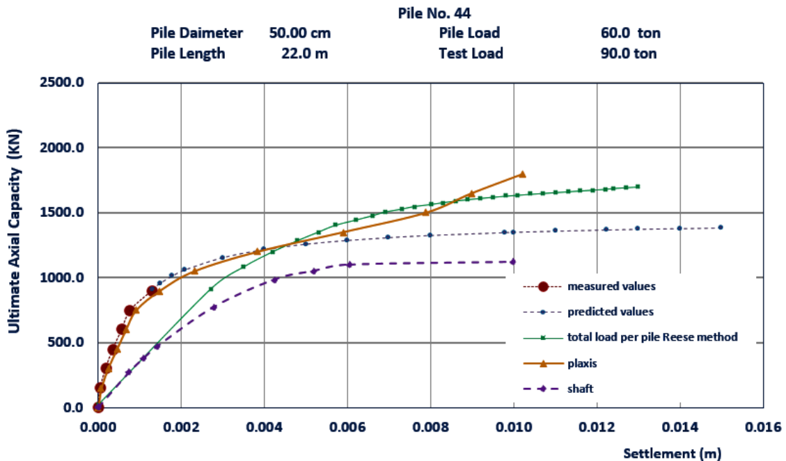
Figure 13: Load- settlement of the pile model No (24) using different methods in a site at Samannoud city.
