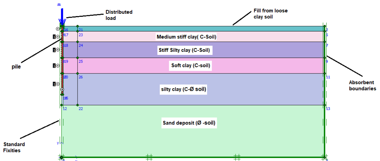
Figure 6: The geometry for 2D PLAXIS model.
