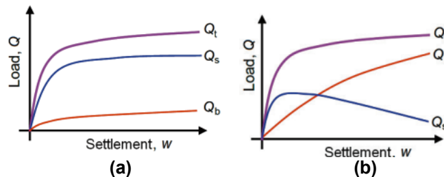
Figure 2: Typical load/settlement curves for compressive load tests: (a) Behavior of friction pile; (b) Behavior of end-bearing pile under compression loading.
