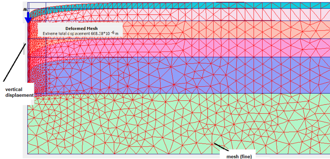
Figure 7: The deformed mesh for 2D PLAXIS model No (26) after applying load.
