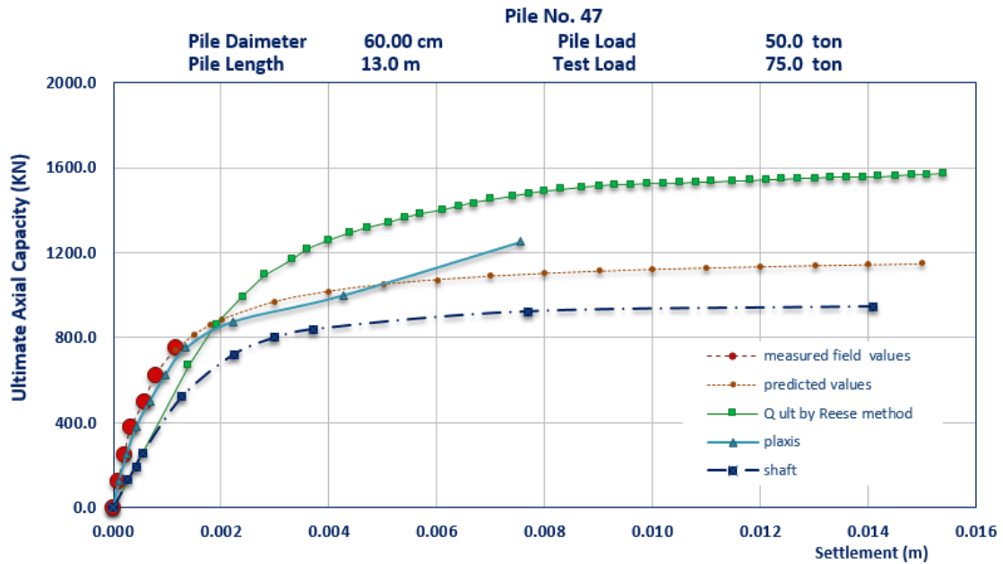
Figure 14: Load- settlement of the pile model No (26) using different methods in a site at Kafr-Elzayat city.
