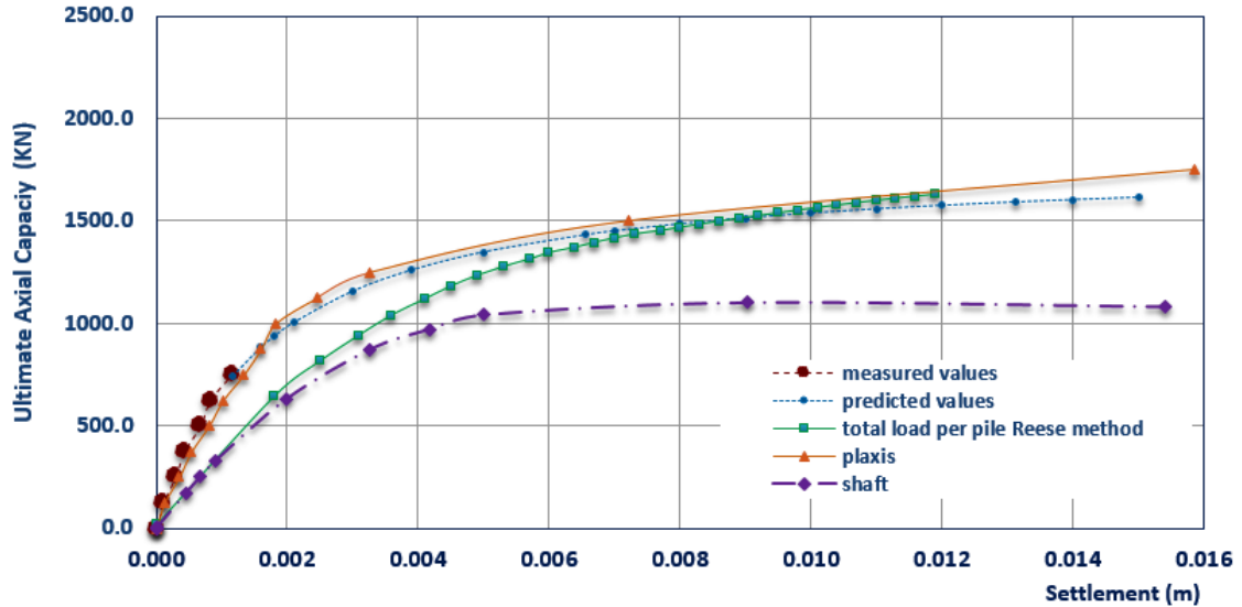
Figure 10: Load settlement behavior of the pile model No (13) using different methods in a site at Al-Mahalla Al- Kubra city.
